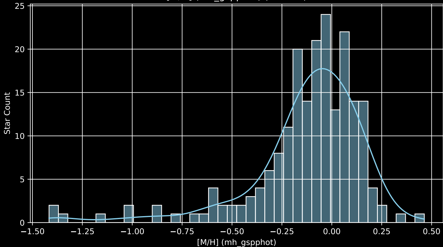
APOGEE DR17 Field: [173-12 [M/H] (mh_gspphot) (n= 203)
