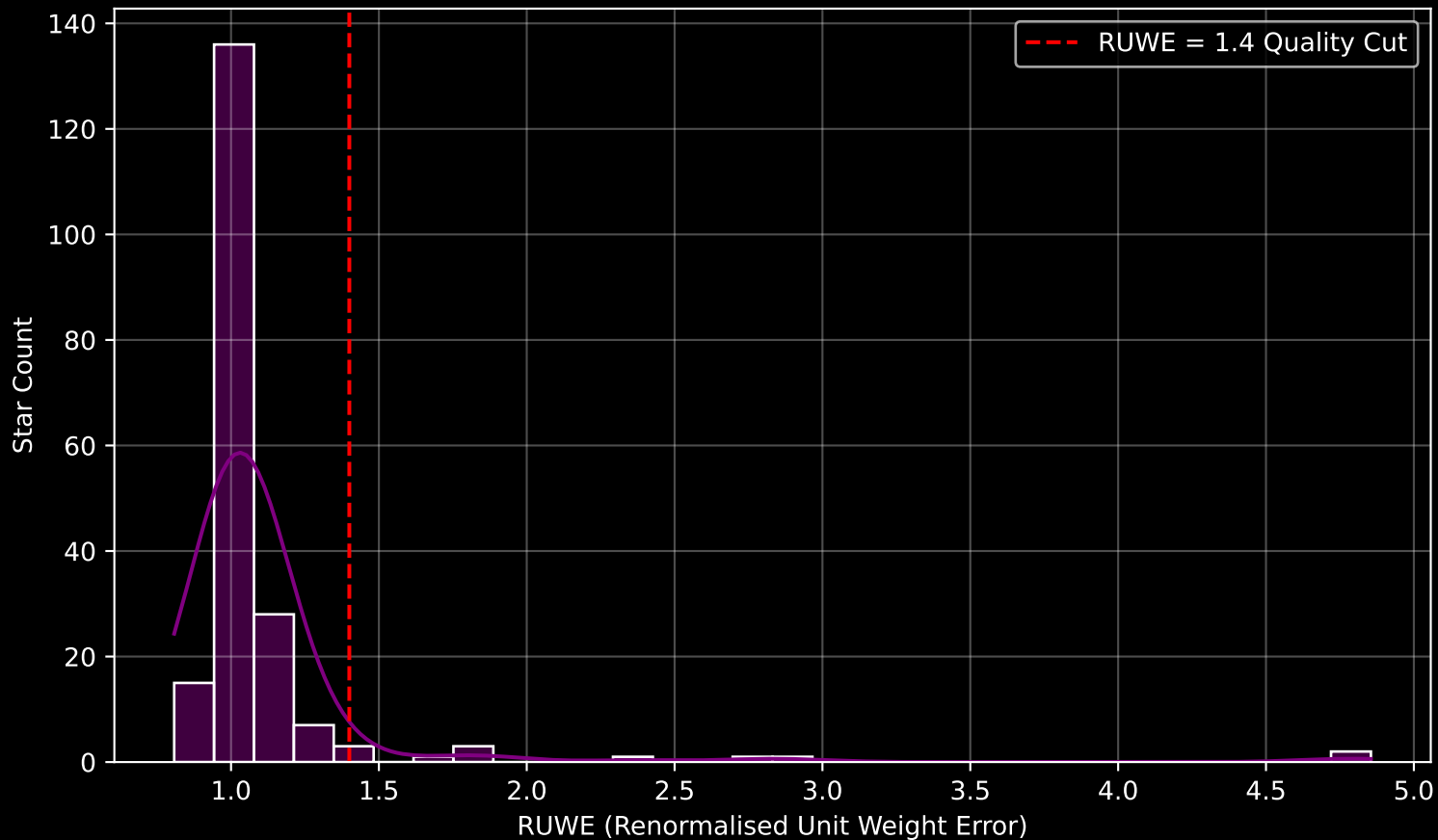
GAPOGEE DR17 Field [173-12] RUWE Distribution (n= 198)
