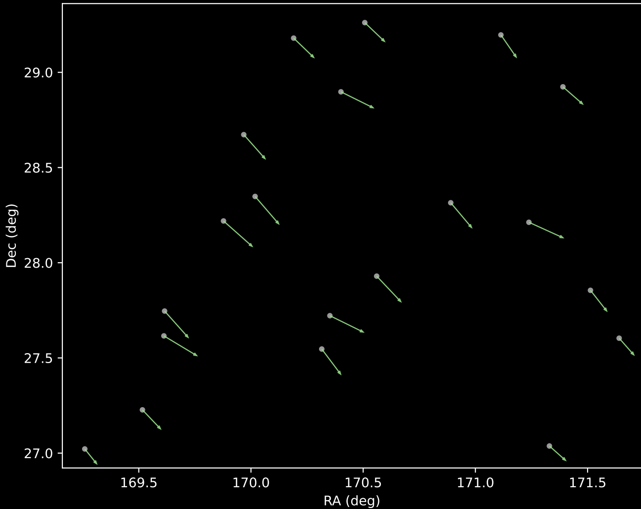
APOGEE DR17 Cluster 5 Proper Motion Vectors (n=20)
