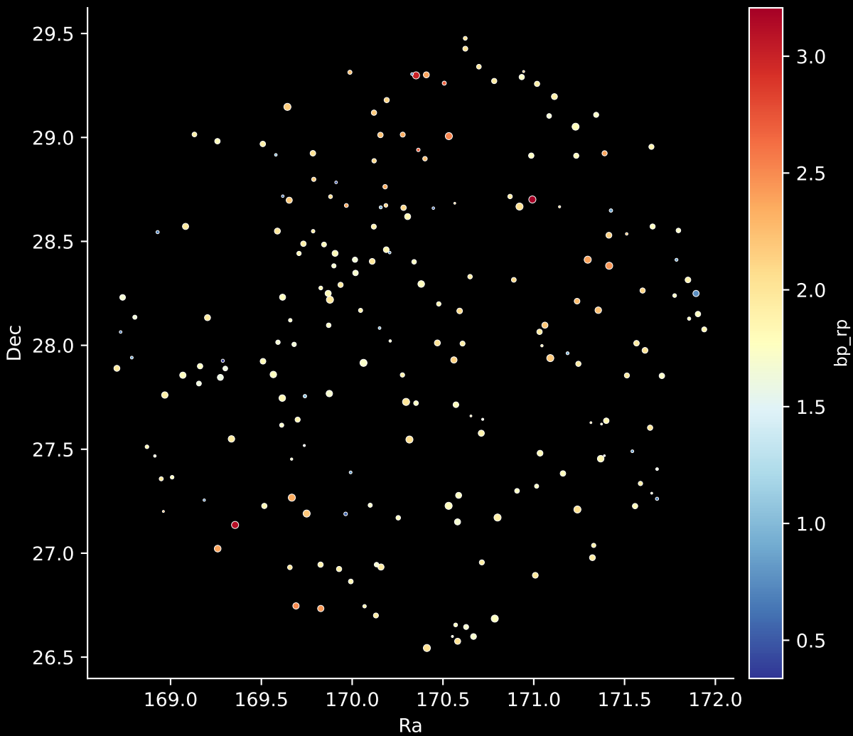
APOGEE DR17 Field: [173-12] Stars: 203
