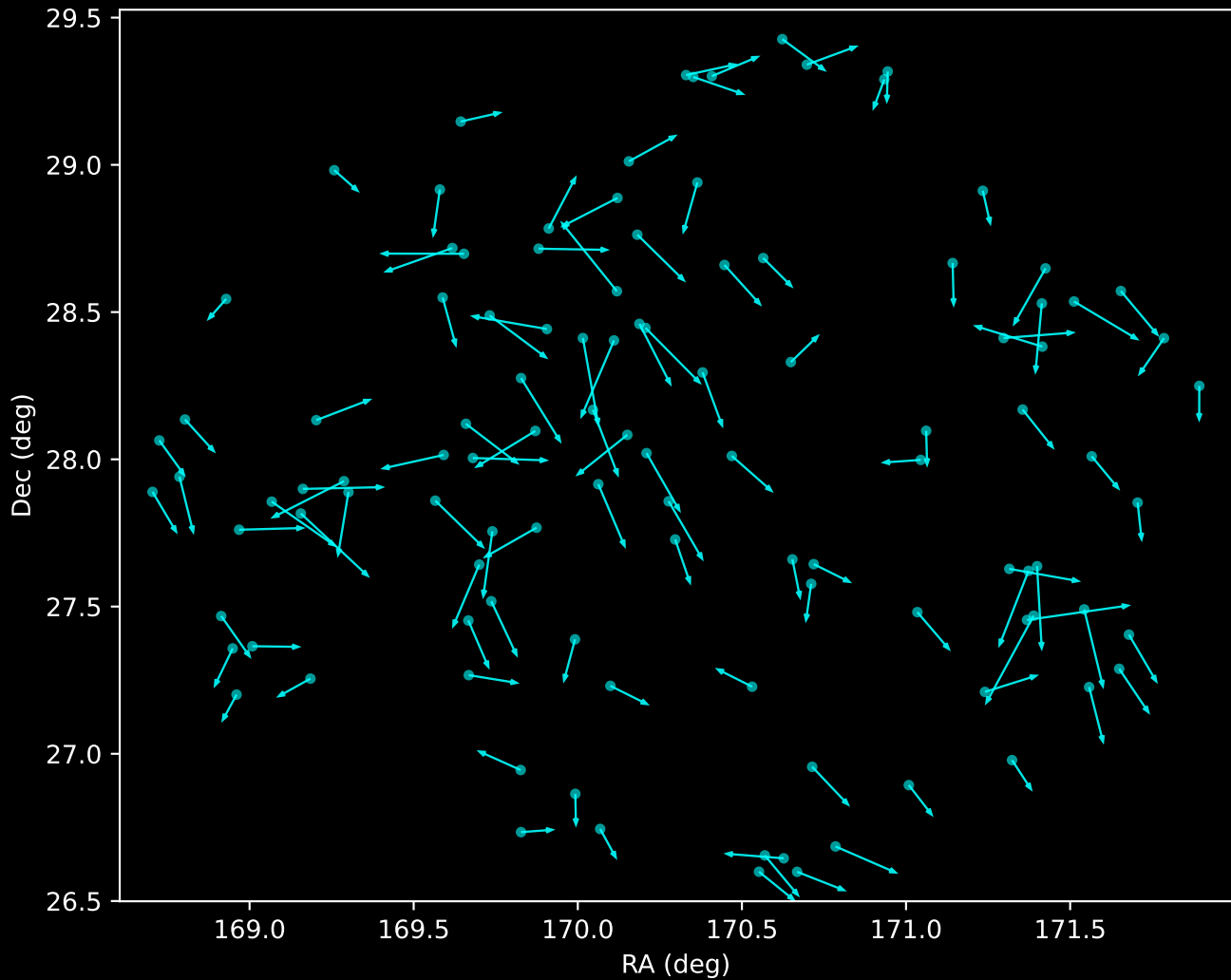
APOGEE DR17 Noise Stream Proper Motion Vectors (n=110)
