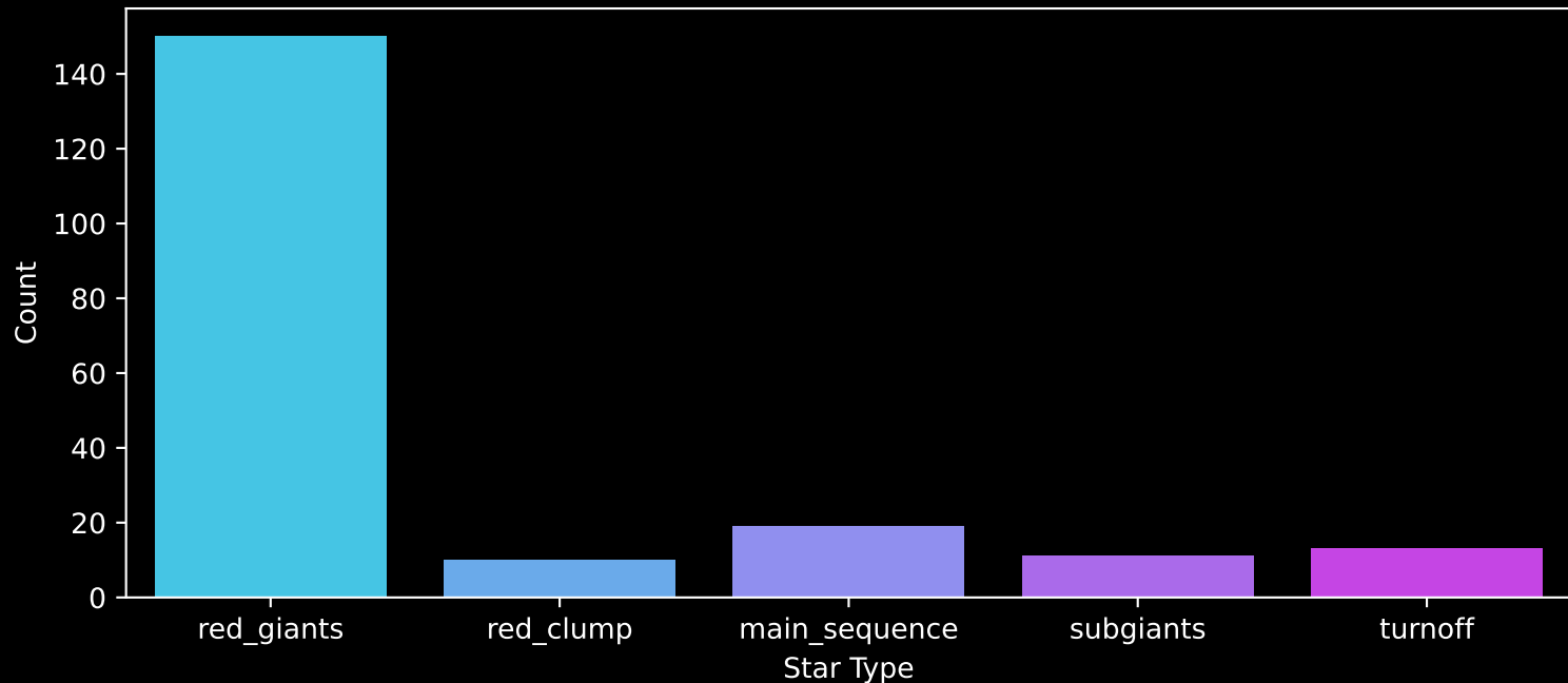
APOGEE DR17 Field: [173-12] Count plot of Star Type
