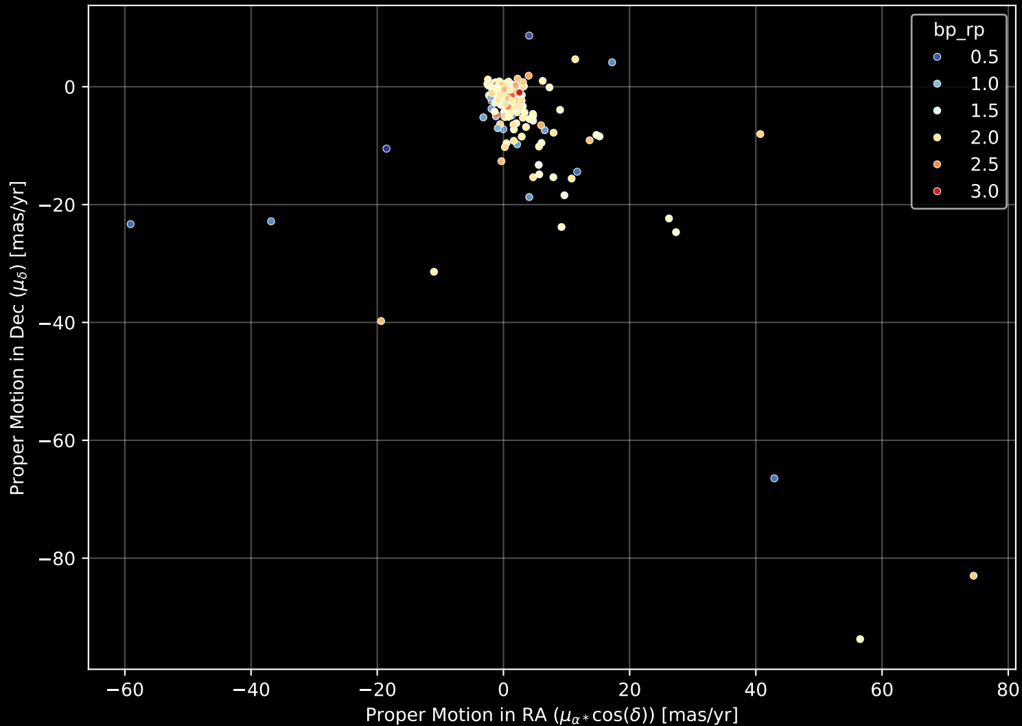
APOGEE DR17 Field: [173-12] Proper Motion Diagram (n= 203)
