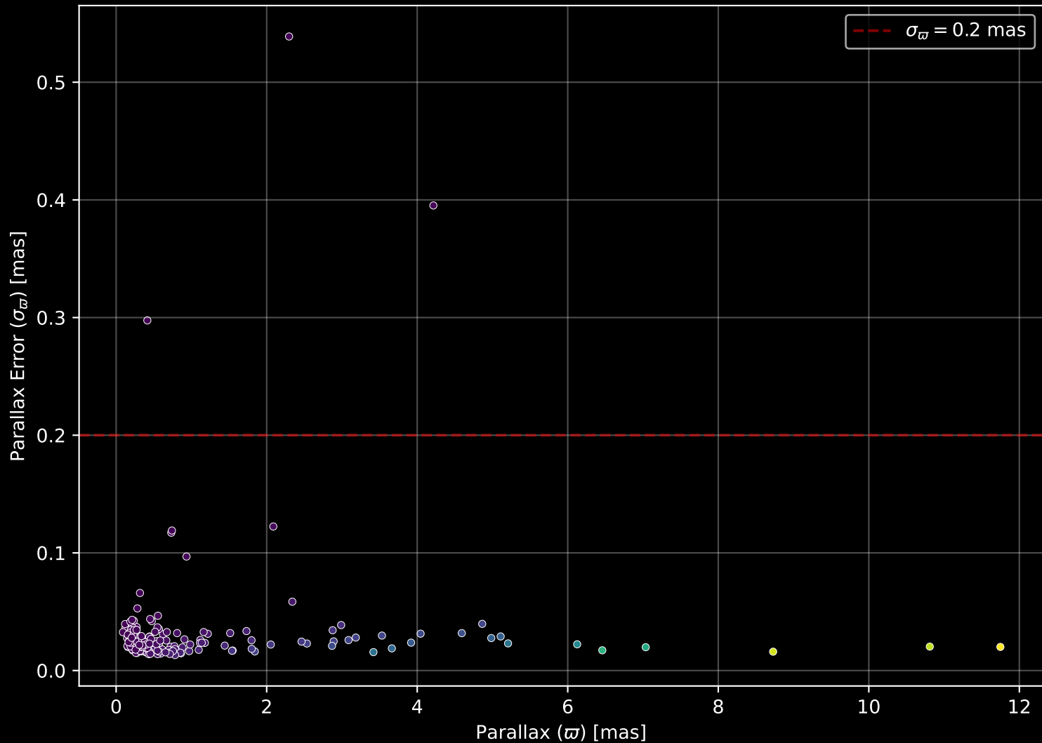
APOGEE DR17 Field: [173-12] Parallax Quality (n= 203)
